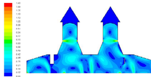
Fig. 7. Velocity spectrum – proposed case
