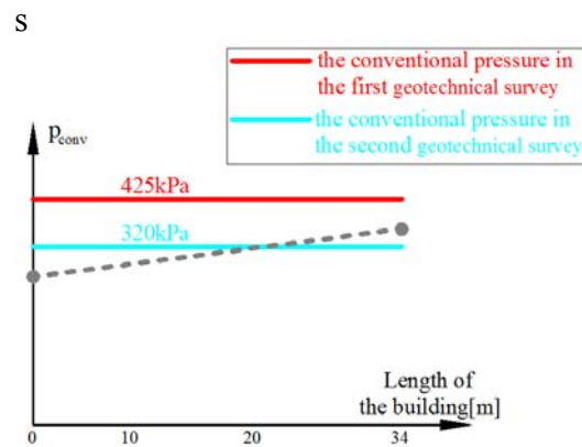
Fig. 4. Bering capacity at the depth of the soil good for foundation the intermediary area
