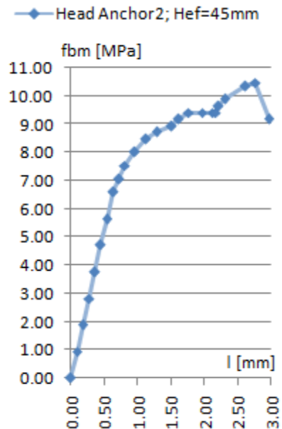
Fig.8. Bond-slip behaviour; mortar ML2
