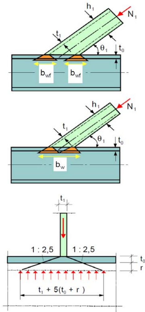
Fig. 3. Model of the chord web failure under compression effect of the diagonal
