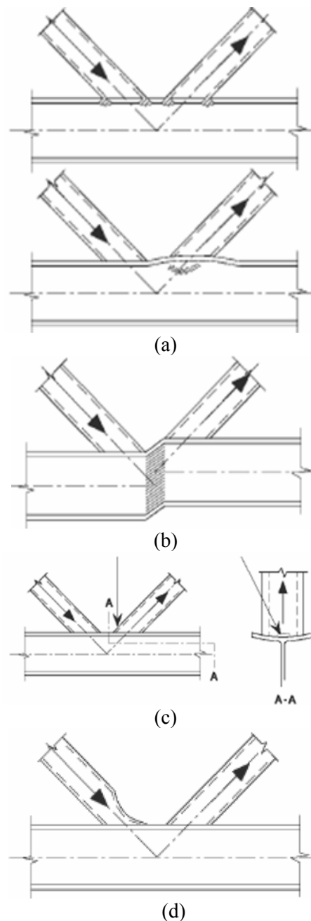
Fig. 2. Failure modes of the joints for truss beams with RHS/CHS diagonals and I or H chord profile type.
