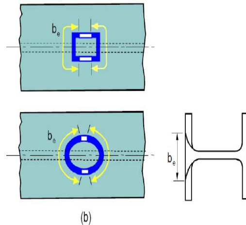
Fig. 7. Model for Failure of the truss element (diagonal) through local yielding and buckling
