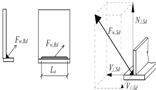
Fig. 6. Simplified method for corner welding design
