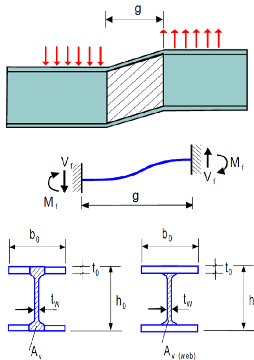
Fig. 4. Model of the chord in share failure
