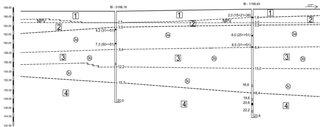
Fig. 2. Geological profile of the terrain 1 and 2. River alluvial sediments(al), 3. Neogene sediments ( ^1M_1^1 ), 4. Peleocen-eocen sediments ( P_c , E_1 )
