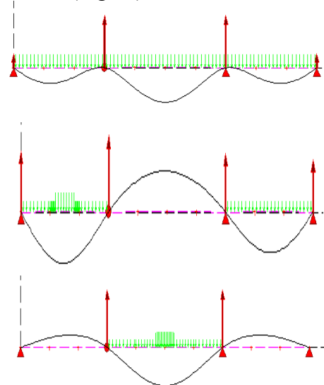
Fig.10. Railway bridge load
