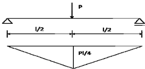
Fig.4 Load concentrated at l/2
