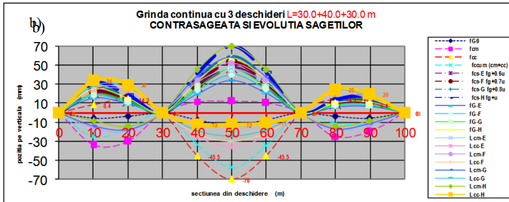
Fig. 12. Precambering and the final deflections: a) situation A-D ; b) situation E-H
