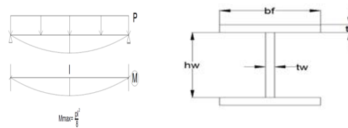
Fig.2 Analysed load cases
