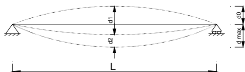
Fig. 1. Vertical deflections of a simple supported beam
