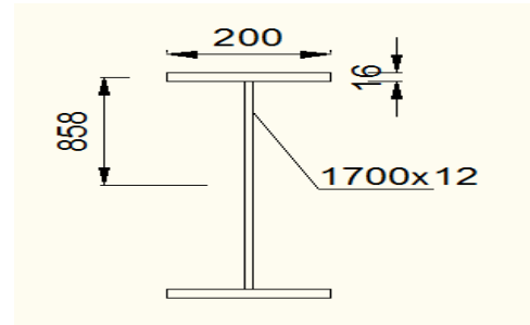
Fig. 3. Predimensioning a railway bridge
